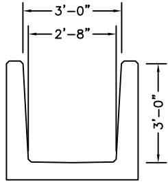
3'-0" WIDE 3'-0" TALL
