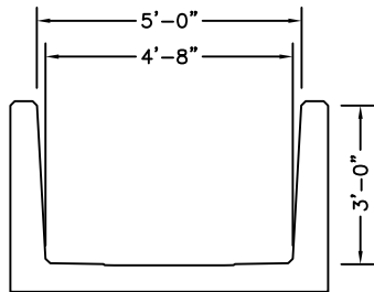
5'-0" WIDE 3'-0" TALL
