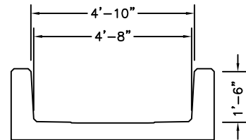
5'-0" WIDE 1'-6" TALL
