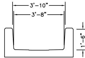
4'-0" WIDE 1'-6" TALL
