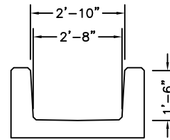
3'-0" WIDE 1'-6" TALL
