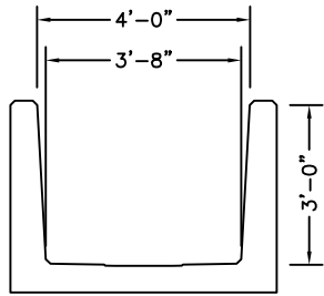
4'-0" WIDE 3'-0" TALL
