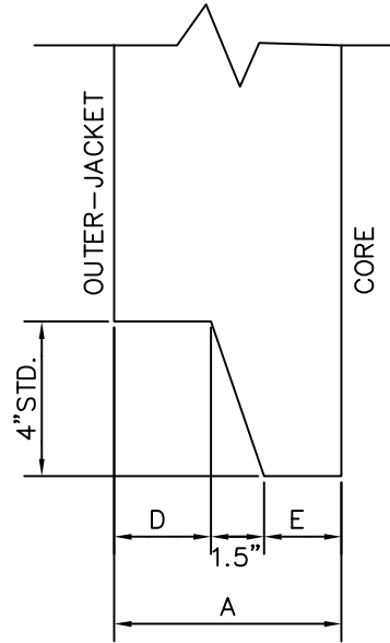
PALLET END
