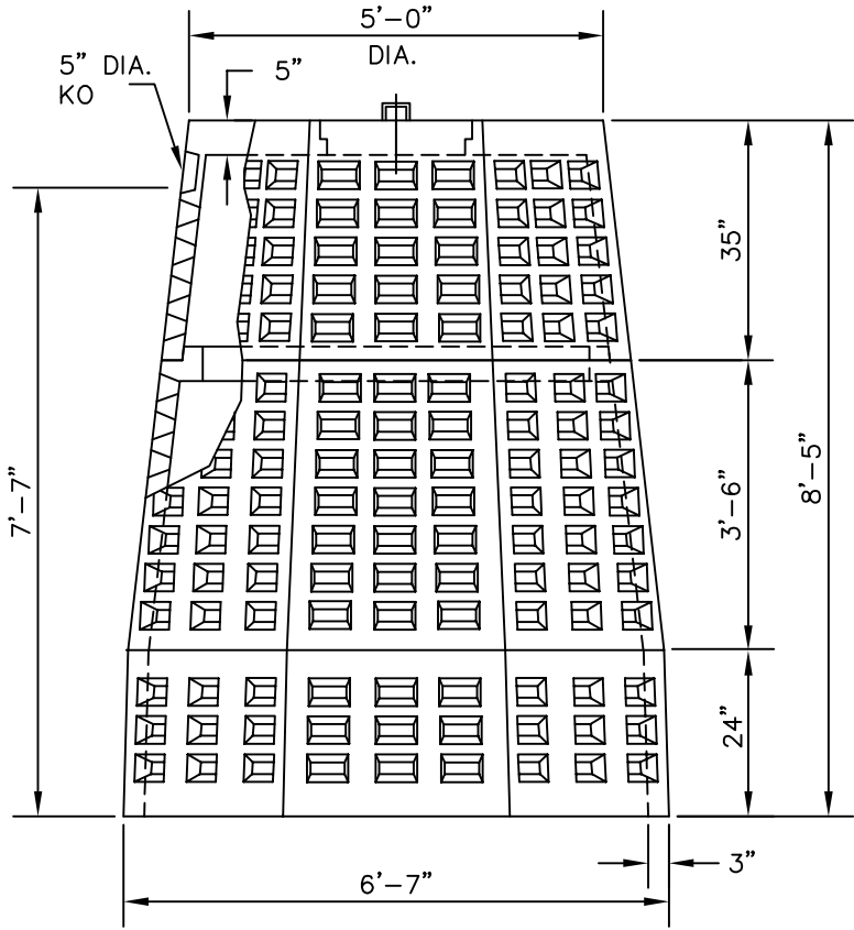
20" DIA. CLEAR OPNG. WITH COVER
